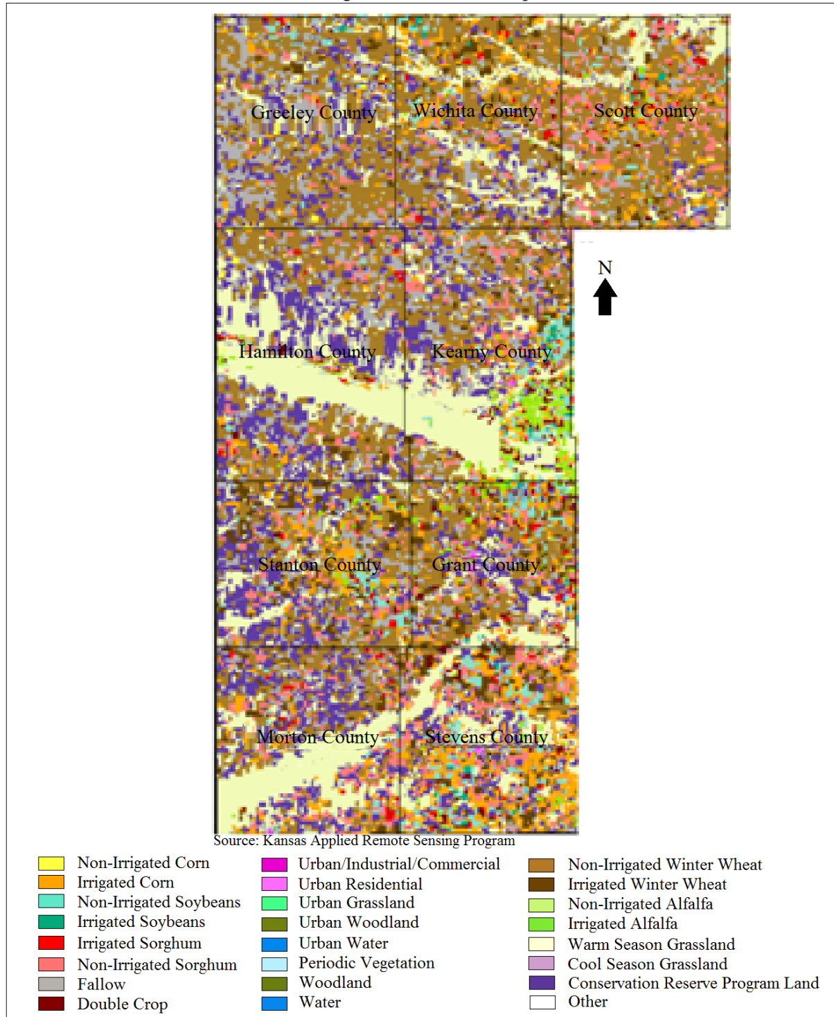
Regional Land Cover Map
