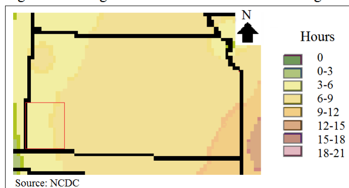
Regional Average Number of Hours with Freezing Rain
