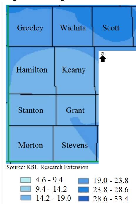
Regional Average Annual Snowfall
